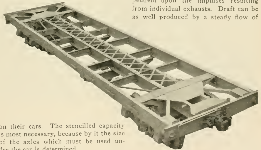
MIDDLETOWN CAR CO.'S STEEL UNDERFRAME FOR BOX CAR.
